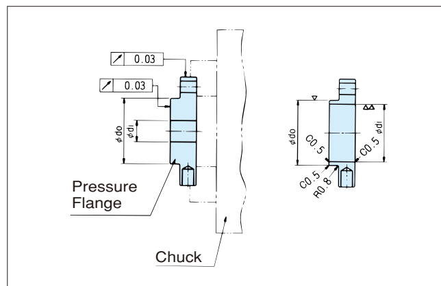
Pressure Flange
